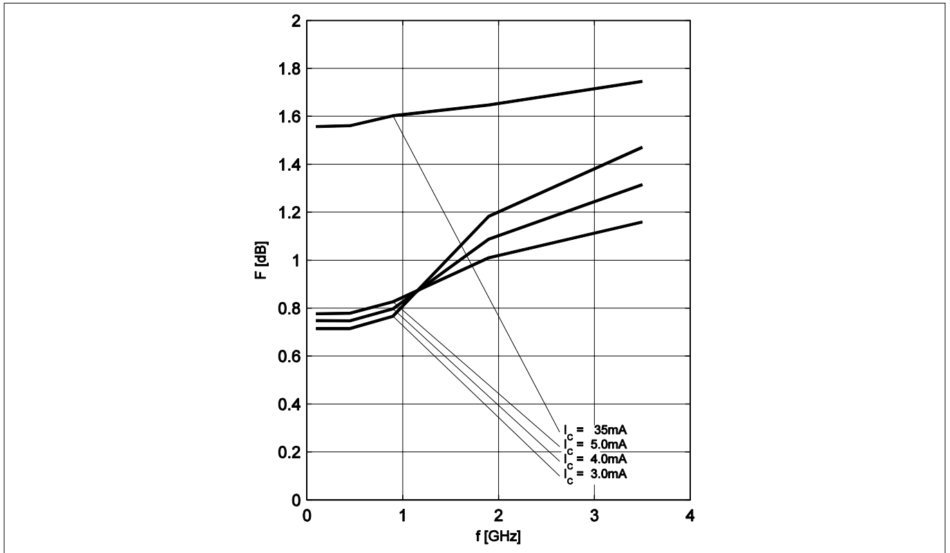
Figure 10 Noise figure NF_{min} = f(f) , V_{CE} = 2V , Z_S = Z_{S,opt} , I_C = \text{parameter}
