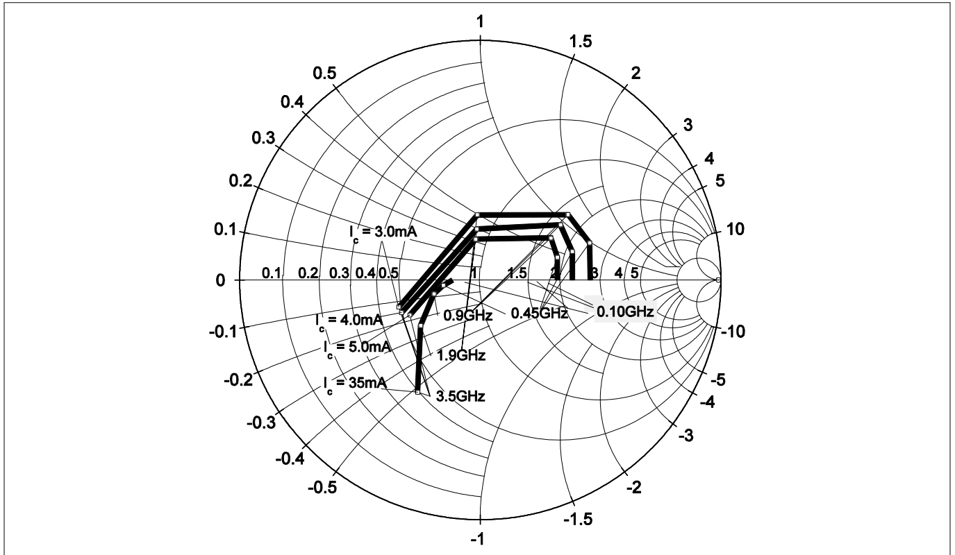
Figure 9 Source impedance for minimum noise figure Z_{S,opt} = f(f) , V_{CE} = 2V , I_C = \text{parameter}
